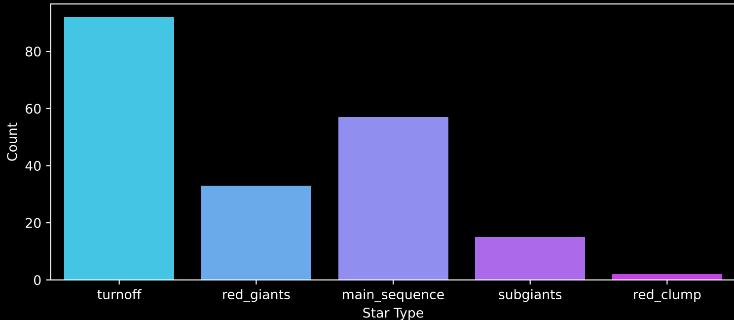
GALAH DR4 Field: [463] Count plot of Star Type
