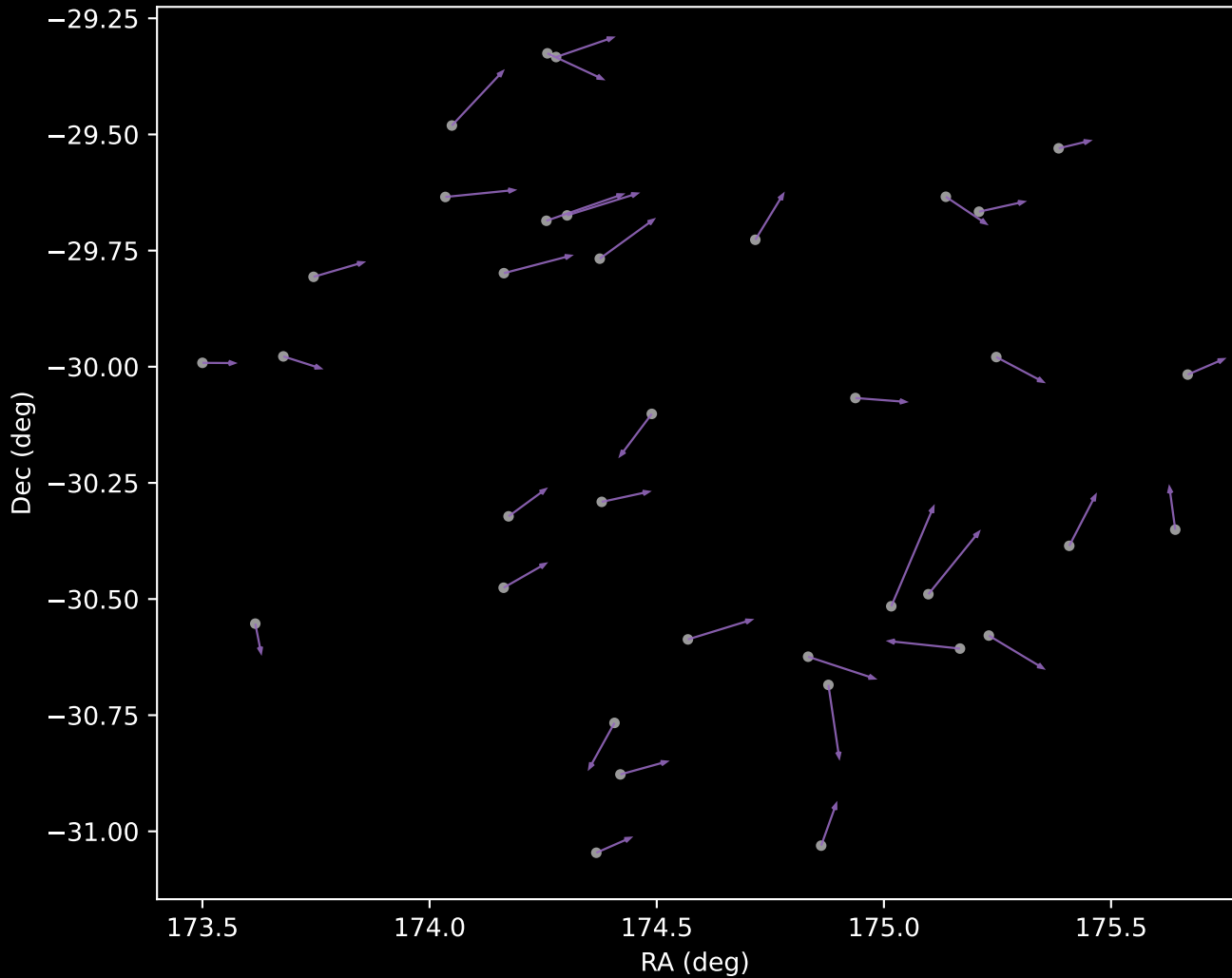
GALAH DR4 Cluster 8 Proper Motion Vectors (n=36)
