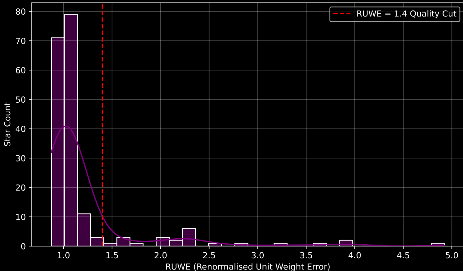
GALAH DR4 Field [463] RUWE Distribution (n= 187)
