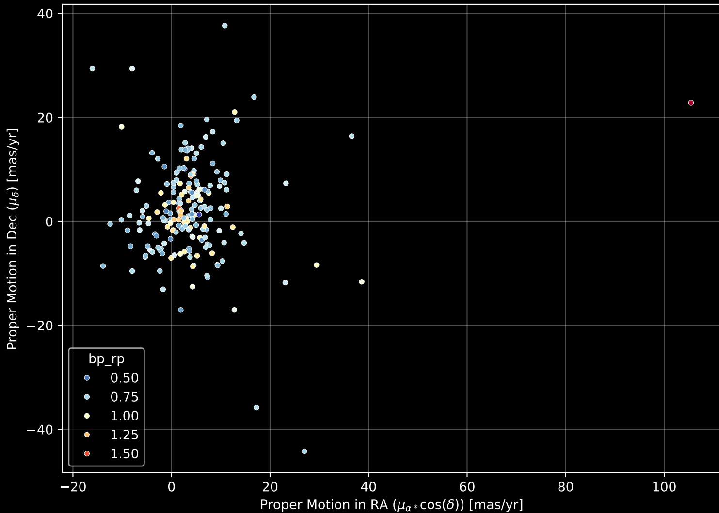
GALAH DR4 Field: [463] Proper Motion Diagram (n= 199)
